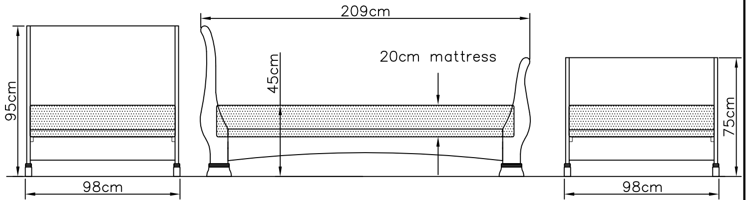
Head end view
