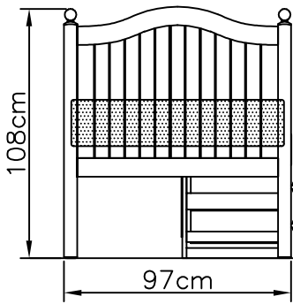
Head end view
