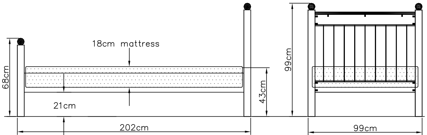
side view
